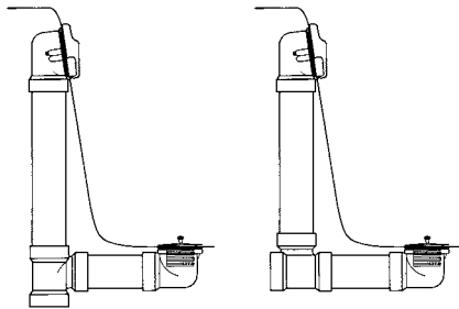
Indirect Bottom Outlet Configuration Indirect Rear Outlet Configuration
