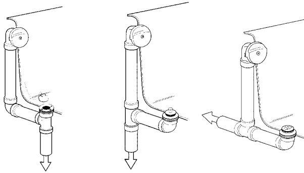
Direct Configuration Indirect Configuration Indirect Rear Outlet Configuration
